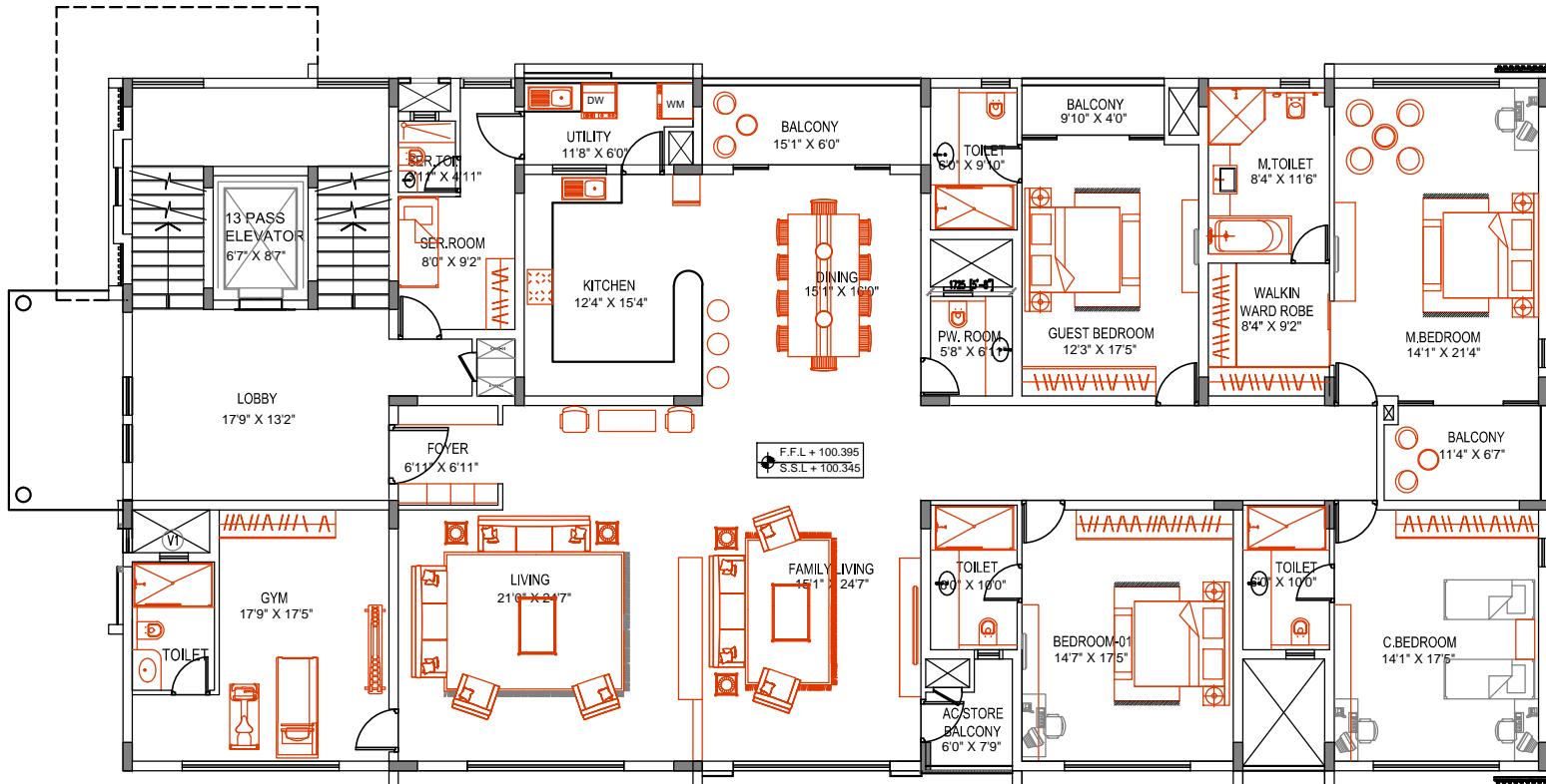
BLOCK K- TYPICAL FLOOR PLAN
